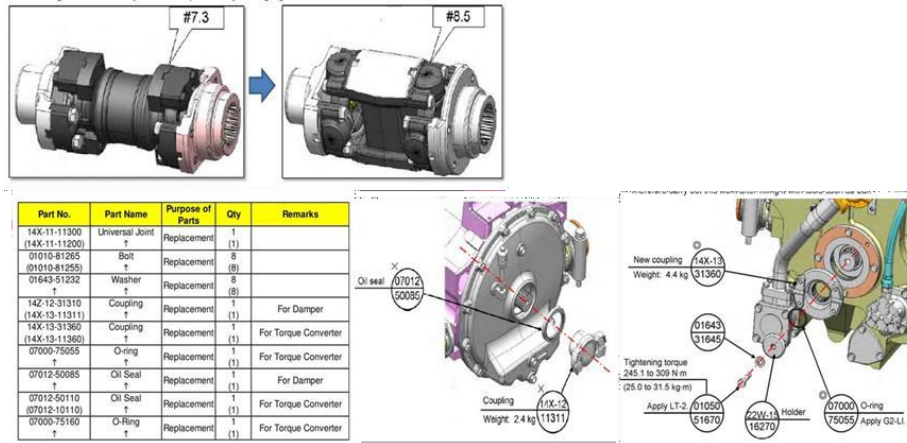
Lampiran 1 : Gambar related part universal joint
